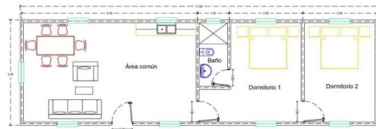
Plan of the new house in the CFC Church property
